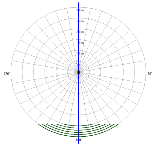
Figure 9. Surf-riding zone (exemplary case)
