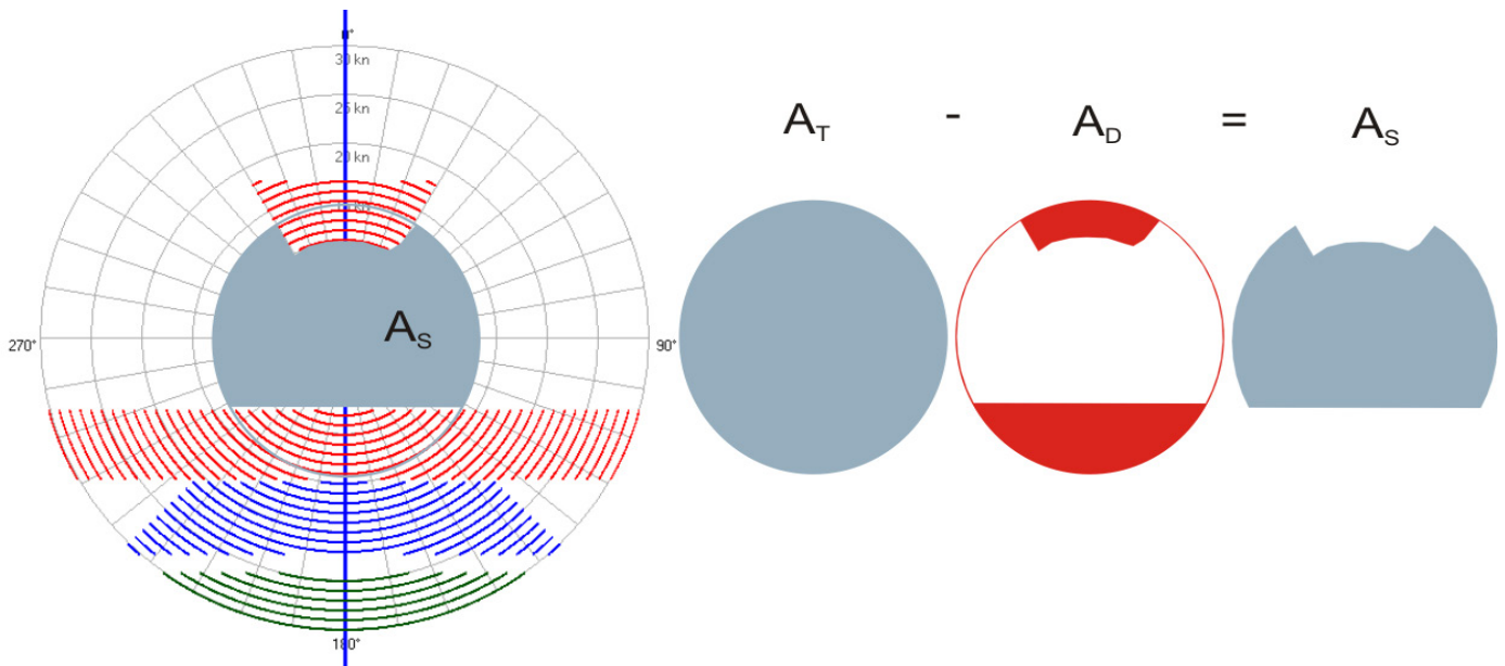
Figure 12. Cumulative graph presenting dangerous zones according to IMO Circ. 1228 (exemplary case)
