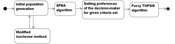
Figure 1. Multicriteria Evolutionary Weather Routing Algorithm (MEWRA)
