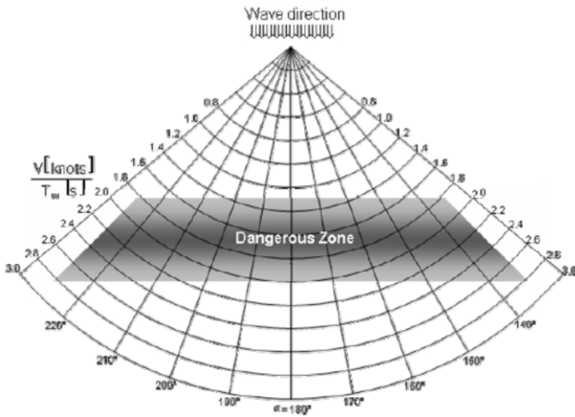
Figure 8. Dangerous zone of successive high wave attack in following and quartering seas (IMO 2007)
