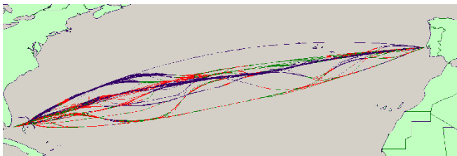
Figure 3. Pareto-optimal set of routes generated by MEWRA for Miami-Lisbon voyage on 2008-02-15 (departure time 12:00 pm)
