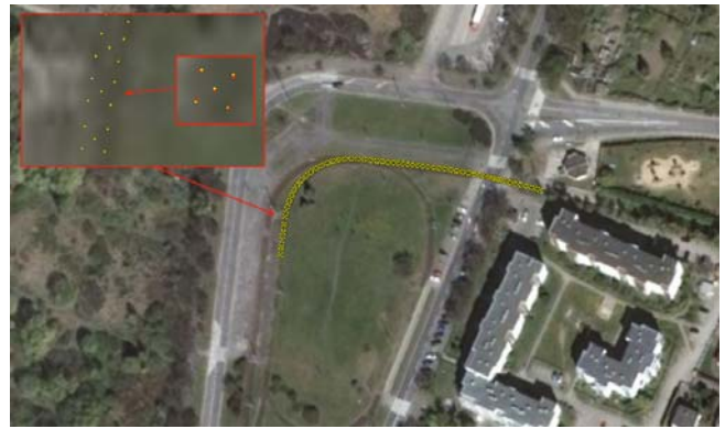
Figure 6. Aligned recording results for a selected section of the tramway track loop in Gdansk – source: prepared by the authors
