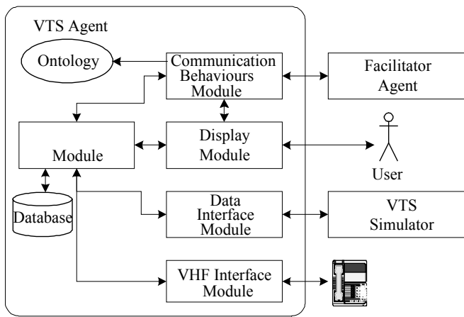
Fig. 2. VTS Agent Structure
