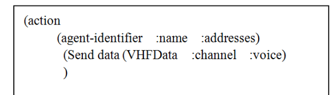
Fig. 4. Structure of message in "update inform" action
