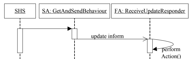
Fig. 3. Time sequence of message from VTS Agent to FA
