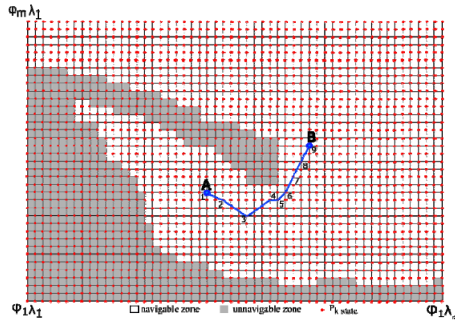
Figure 2. Descritized chart with constant granularity of area with example of route from start point A to finish point B with 32 possible movements of a sailing vessel from each point P_k , illustrated are 9 points P_k , where in point designed by 7, 8, 9 is course
