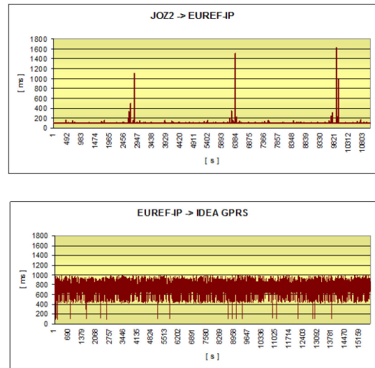
Fig. 5. Packet acquisition time from Józefosław to the EUREF-IP broadcaster as well as from the broadcaster to the user
