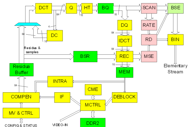
Figure 1. Block diagram of the H.264/AVC encoder
