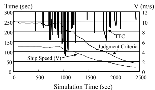
Fig. 5. Calculation results of TTC
