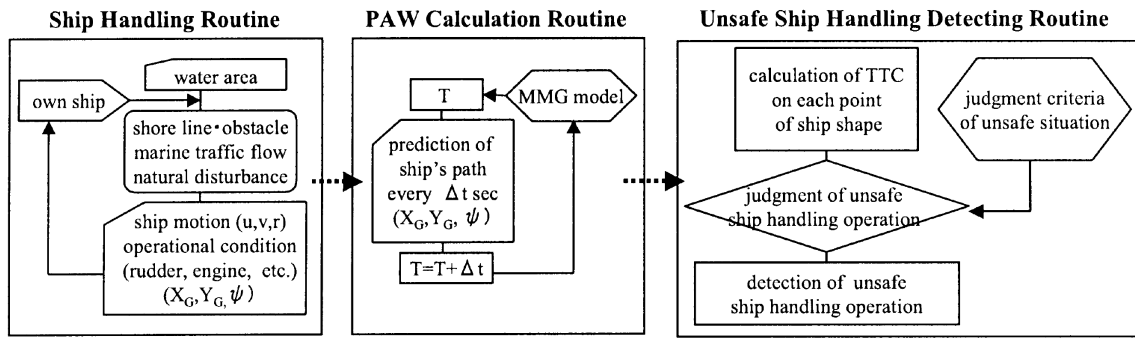
Fig. 3. Flowchart of detection procedure
