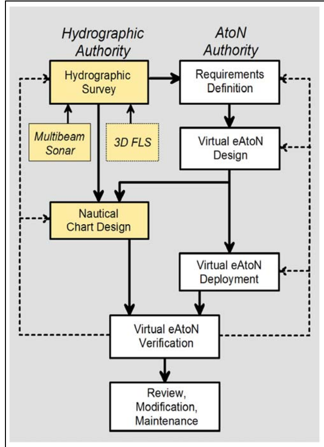
Figure 2. Virtual eAtoN life cycle representing roles of national hydrographic and AtoN authorities.
