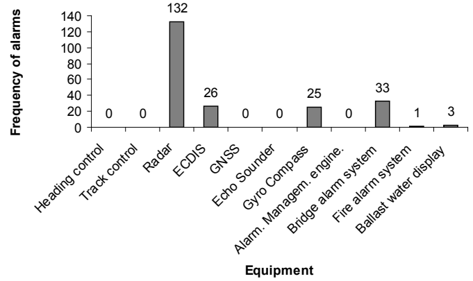
Fig. 3. Frequency of alarms per device
