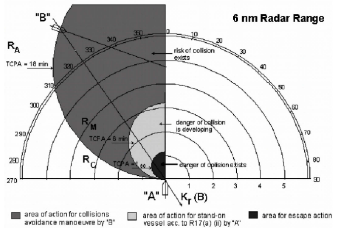
Fig. 6. Application of the risk model to an encounter situation on crossing courses under conditions of good visibility
