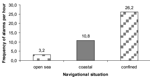
Fig. 2. Average frequency of alarms depending on sea areas for a voyage of a passenger vessel
