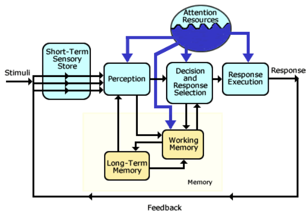
Figure 1. Model of human information processing
