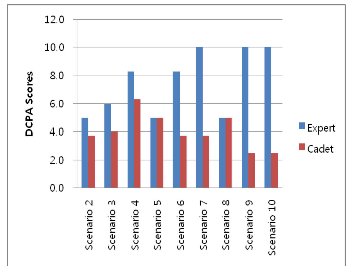
Figure 6. Comparison of the DCPA scores by scenarios
