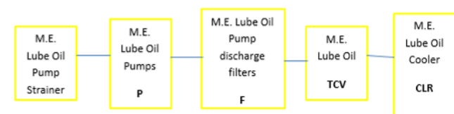
Figure 3. Detailed RBD for M.E. Lube Oil system, with all system components
