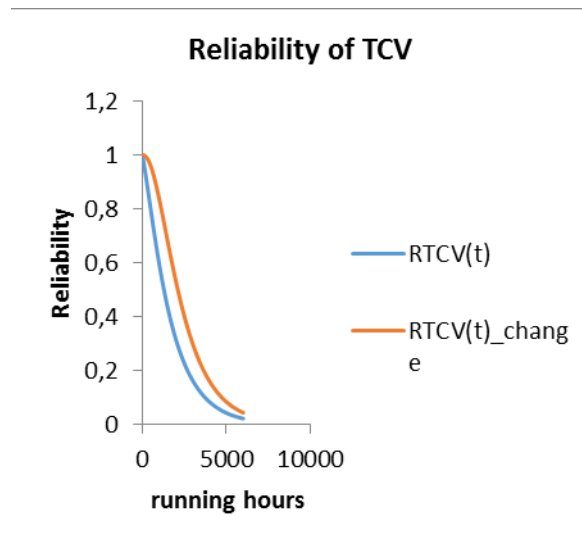
Figure 11. Change in reliability by addition of Temp Cont Valve
