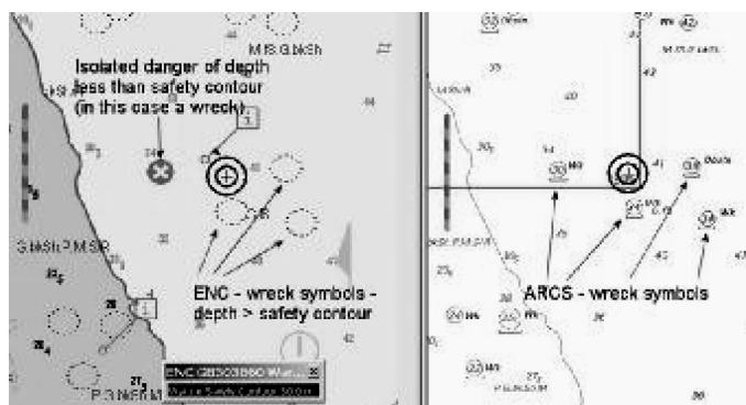
Fig. 1. An example of the use of the Isolated Danger symbol on an ENC
